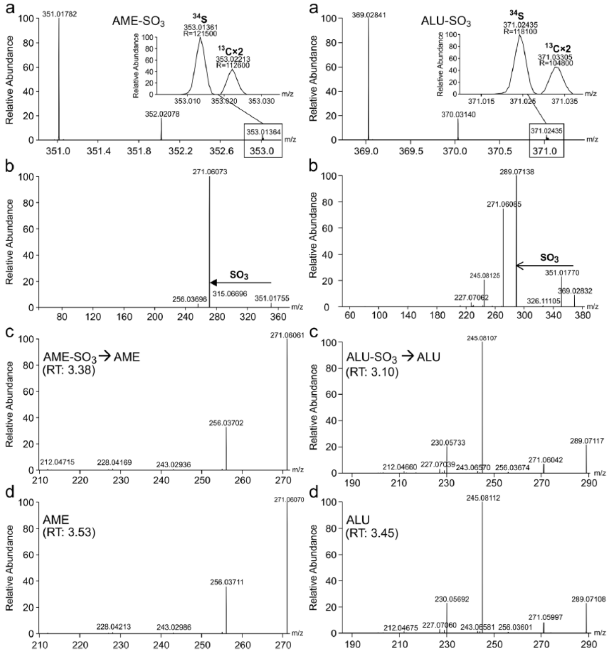
Figure 31- A) MS spectra including isotope pattern at high resolution showing the fully resolved 34 S peak as evidence for sulfoconjugation of the known metabolite AME and the new metabolite ALU-SO 3 . B) MS 2 spectra for each metabolite confirming the neutral loss of SO 3 . C) MS 3 spectra for the sulfoconjugated version of each metabolite showing the fragment ions of the in source generated 'free' metabolite. D) MS 2 spectra for 'free' versions of both metabolites showing the same fragmentation patterns as the MS 3 of the sulfoconjugated metabolites.
