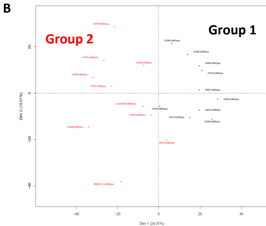
Figure 15- PCA plots of metabolomics data generated in negative ionization mode (A) and positive ionization mode (B) for 20 randomly selected samples. Samples are coloured by their previous K-means clustering assignment (Figures 13 and 14 )
