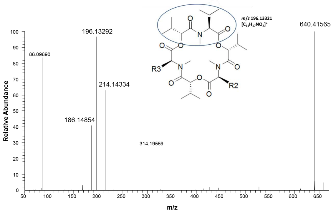
Figure 36- MS 2 spectrum of enniatin B in positive ionization mode, showing the common 196.13321 product ion
